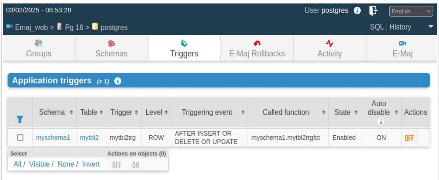
Figure 14 – Application triggers list.
