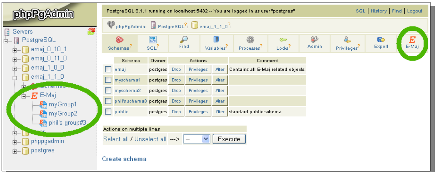
Figure 1 – Connection to a database where E-Maj is installed.
